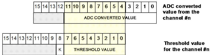
Fig. 2.5: Zero suppression (Bit 8 of Bit Set 2 Register = 0, default setting)
