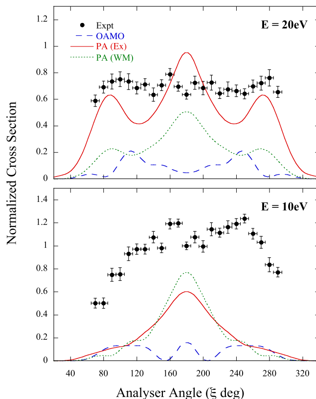
Figure 5. Experimental and theoretical TDCS for the HOMO of \text{SF}_6 for the perpendicular geometry. Incident energies of 40 and 20 eV above the ionisation potential were used, corresponding to outgoing energies of 20 and 10 eV respectively, as indicated on the respective plots. Three theoretical predictions are shown for all energies. Calculations using the proper average (PA) over molecular orientations and the post collision interaction (PCI) treated exactly (Ex) are shown in the solid red curve, while the green dotted curve shows results in which the Ward–Macek approximation (WM) has been used to represent PCI. The calculation using the orientation averaged molecular orbital (OAMO) approximation and exact PCI is the blue dashed curve. The experimental and theoretical data have been normalized to the coplanar data at \xi_1 = \xi_2 = 90^\circ , or \phi = 180^\circ , as discussed in the text. The TDCS must be symmetric around \phi = 180^\circ , and so the small variations in the data for E = 10 eV are attributed to the low coincidence yields that were obtained at this energy.
