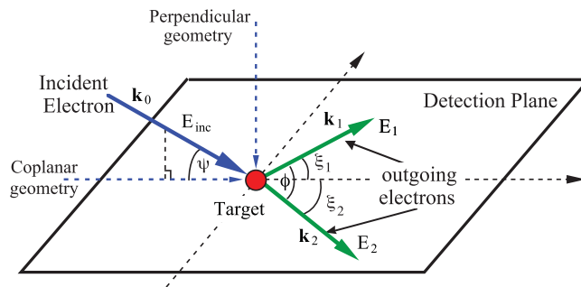
Figure 1. Schematic of the experimental geometries used in this study. A coplanar geometry ( \psi = 0^\circ ) is defined when the incident electron momentum \mathbf{k}_0 lies in the detection plane defined by \mathbf{k}_1 and \mathbf{k}_2 . The analyzer angles ( \xi_1 and \xi_2 ) are measured with respect to the projection of the incident electron momentum \mathbf{k}_0 in this plane, as shown. The perpendicular geometry is accessed by moving the electron gun to an angle \psi = 90^\circ . In this geometry the only relevant angle is the mutual angle \phi = \xi_1 + \xi_2 between the two analyzers.
