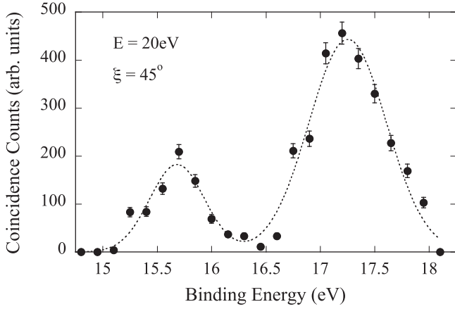
Figure 2. A typical coincidence binding energy spectrum obtained for SF 6 . The experimental data is shown, and the dotted curve is a fit of two Gaussians to the data. This spectrum was measured in a coplanar geometry with outgoing electron energies E = 20 eV at an angle \xi = 45^\circ . The peak at lower energies (15.7 eV) is due to the highest occupied molecular orbital (HOMO), that at the higher energy (17.2 eV) is attributed to the next highest occupied molecular orbitals (NHOMO) and NHOMO-1 orbitals that are almost degenerate. The data demonstrate that good separation has been achieved using the current experimental energy resolution, so that the TDCS data can be attributed to the HOMO only.
