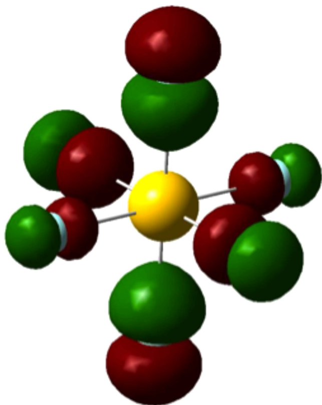
Figure 4. A representation of SF 6 HOMO wavefunction. The individual p-type orbitals are all centered on the fluorine nuclei.
