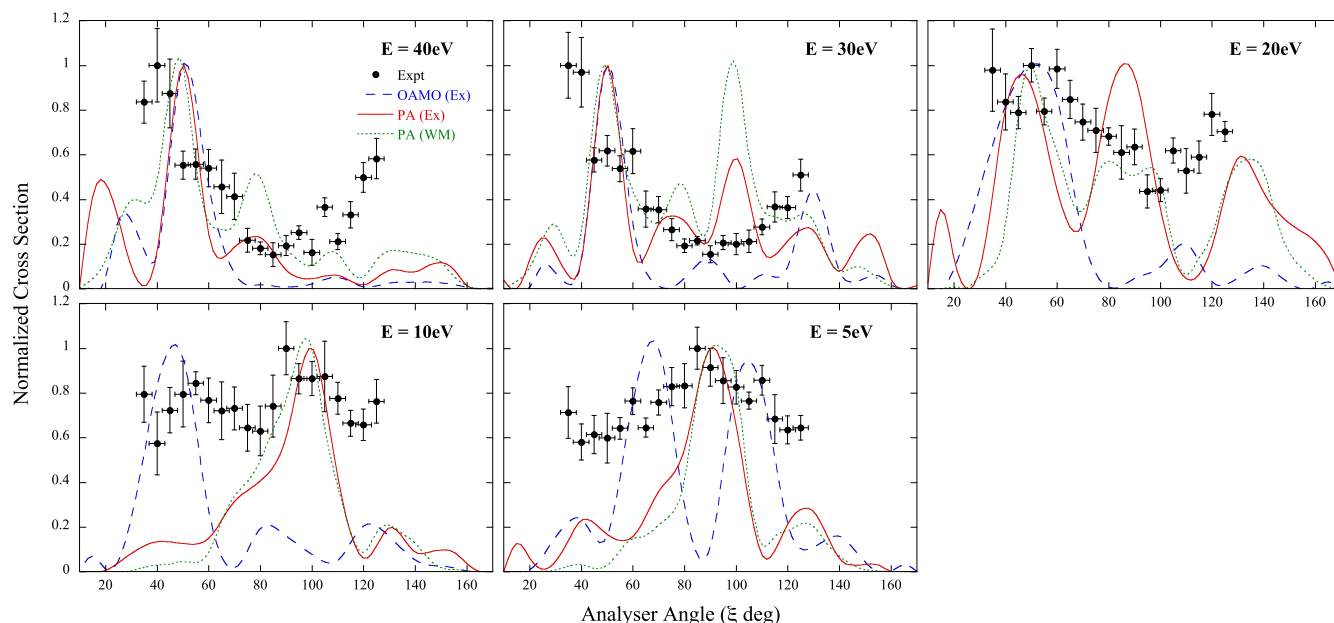
Figure 3. TDCS from the HOMO of sulphur hexafluoride for coplanar symmetric kinematics. Incident energies ( E_0 ) of 10–80 eV above the ionisation potential (15.7 eV) were used. The energies of the outgoing electrons ( E_1 and E_2 ) satisfy the conservation of energy such that E_0 + \text{IP} = E_1 + E_2 . The energies shown on the respective plots are those of the outgoing electron where E_1 = E_2 = E , as defined by the doubly symmetric geometry employed. The experimental data (dots) and results from the molecular three-body distorted wave approximation (lines) are shown. Calculations using the proper average (PA) over molecular orientations and the post collision interaction (PCI) treated exactly (Ex) are shown in the solid red curve, while the green dotted curve shows results in which the Ward–Macek approximation (WM) has been used to represent PCI. The calculation using the orientation averaged molecular orbital (OAMO) approximation and exact PCI is the blue dashed curve. The experimental and theoretical data have been independently normalized to unity at the highest intensity for each energy.
